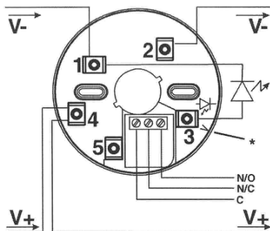
Fig. / Abb. 2b ECO1000BRELx
