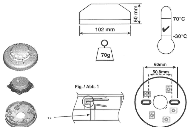
Fig. / Abb. 2a ECO1000B ECO1000DB ECO1000BRx ECO1000DBRx ECO1000BSD ECO1000DBSD ECO1000BRxSD ECO1000DBRxSD
