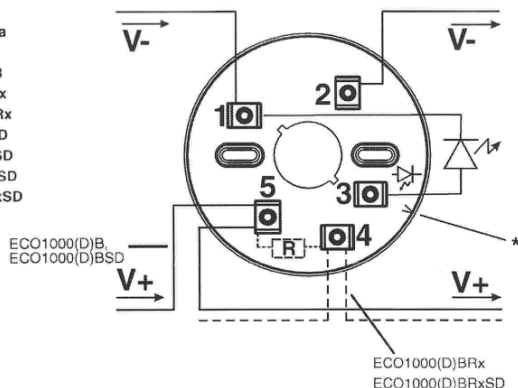
Fig. / Abb. 2b ECO1000BRELx
